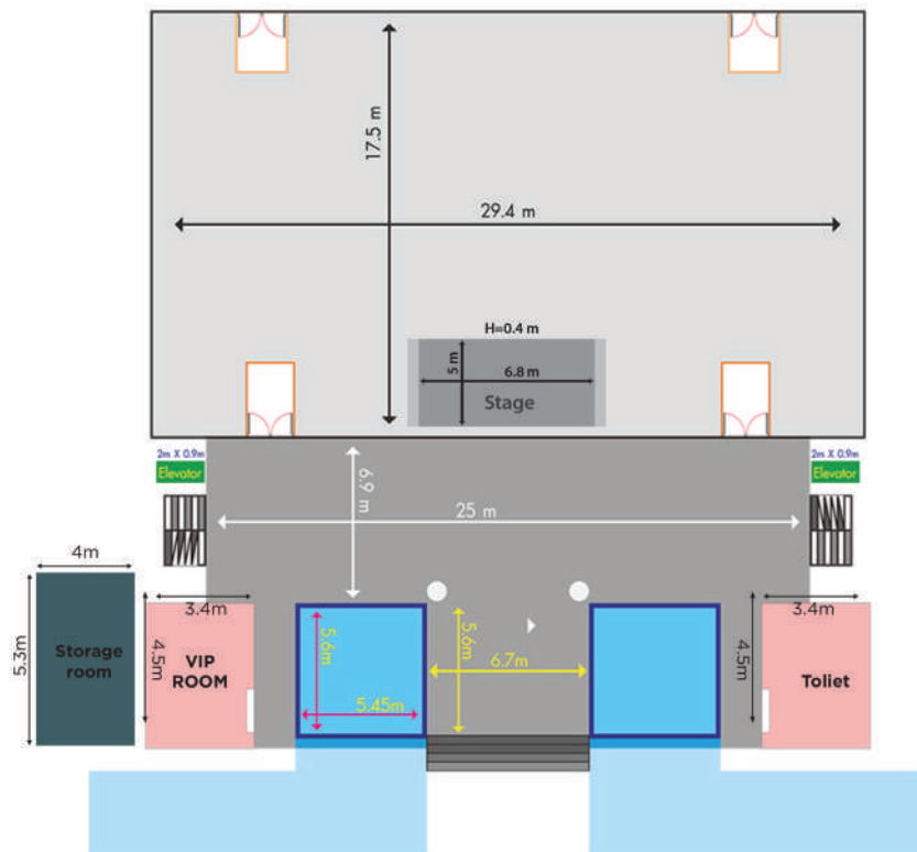
Floor-plan Parisorn Ballroom
